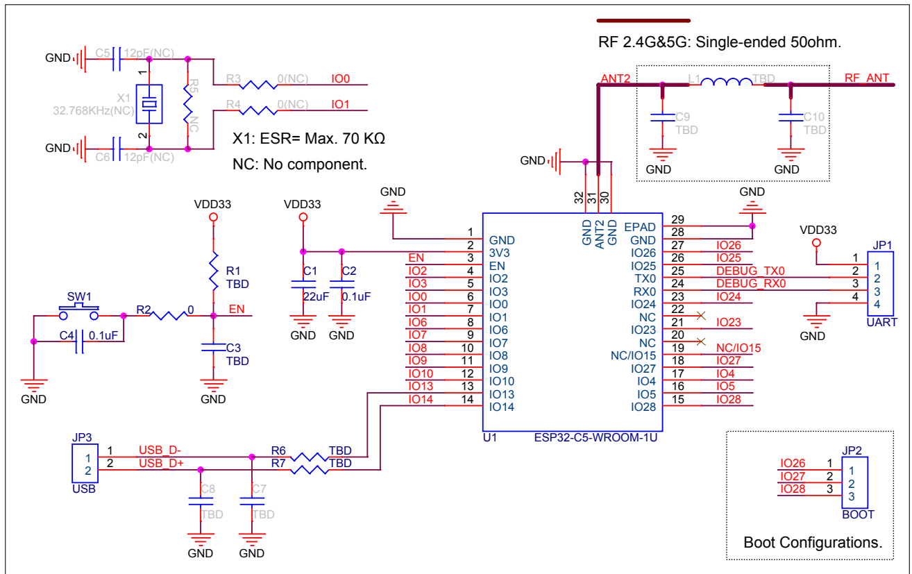
Figure 9-2. ESP32-C5-WROOM-1U Schematics
