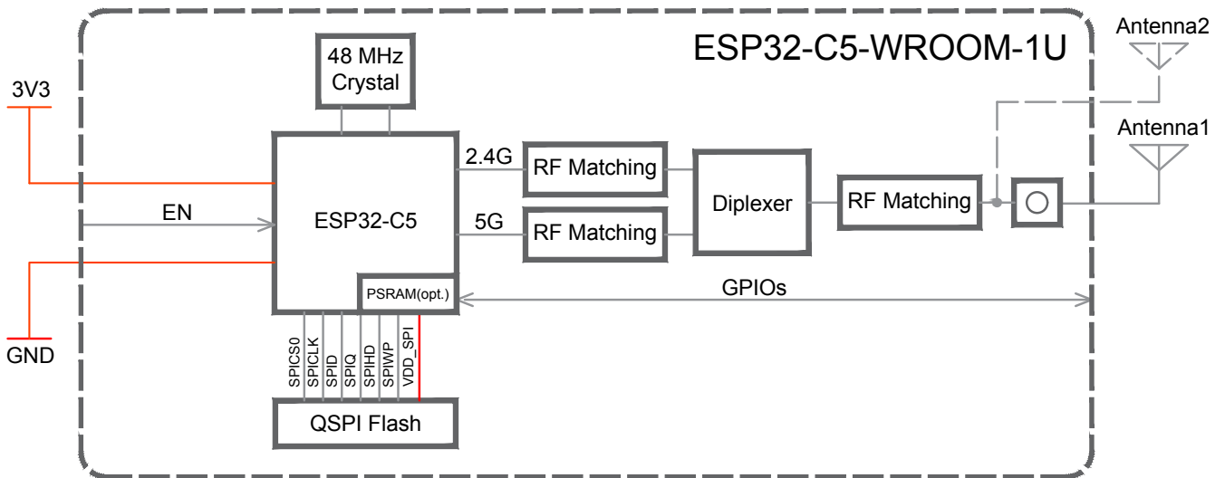
Figure 2-2. ESP32-C5-WROOM-1U Block Diagram
