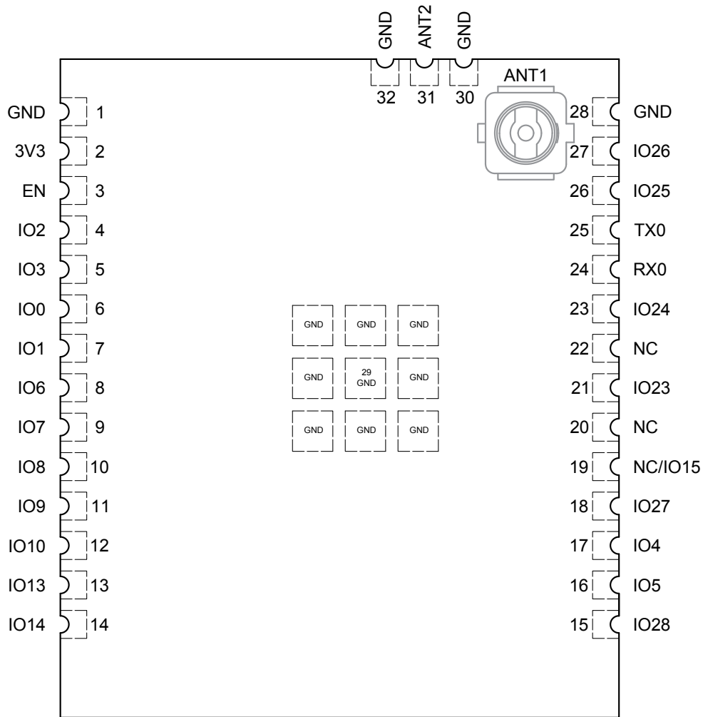
Figure 3-2. ESP32-C5-WROOM-1U Layout (Top View)
