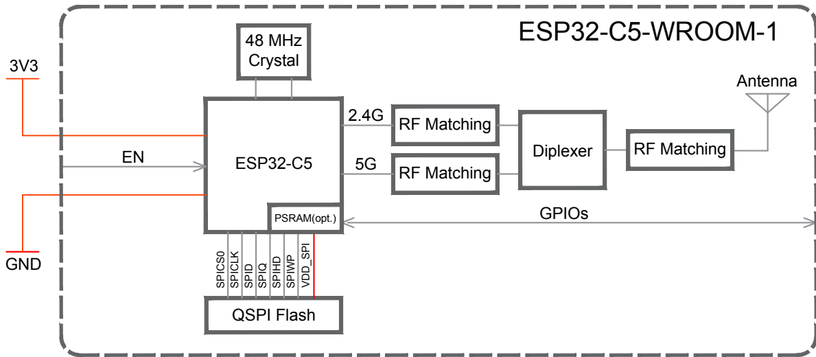
Figure 2-1. ESP32-C5-WROOM-1 Block Diagram
