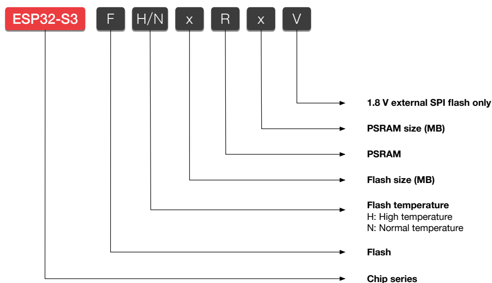
Figure 1-1. ESP32-S3 Series Nomenclature
