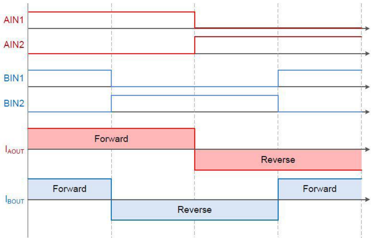
FULL STEP
