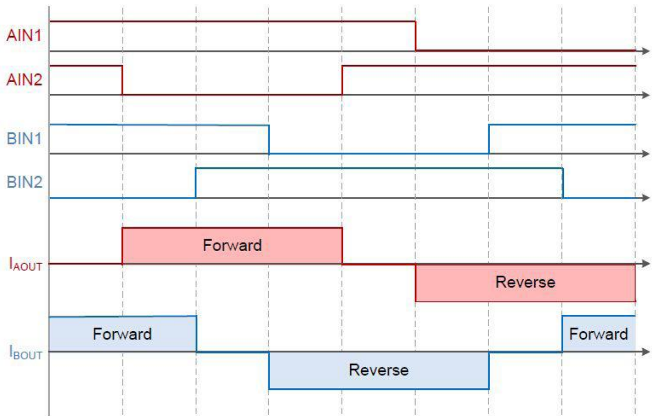
FULL STEP
