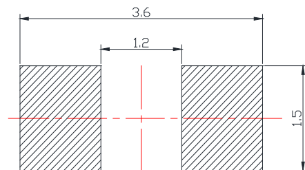
推荐焊盘尺寸 Recommended Soldering Pad
