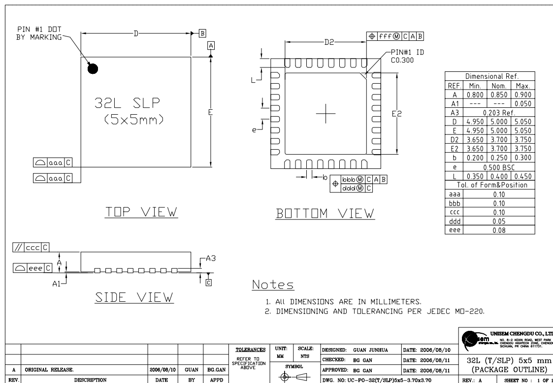
Figure 6-1. ESP8266EX Package
