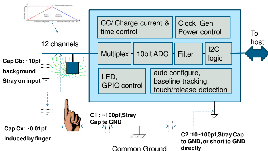
Figure 3. MPR121 Block Diagram and Capacitance Measurement
