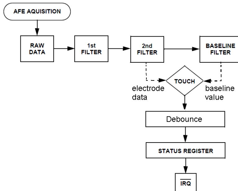
Figure 4. MPR121 Capacitance Measurement
